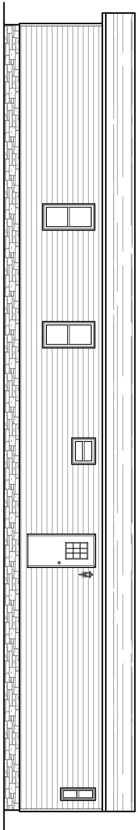
REAR SIDE ELEVATION
