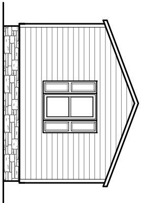
RIGHT SIDE ELEVATION
