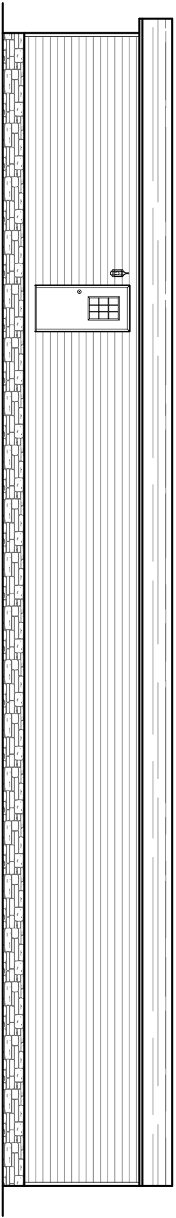
REAR ELEVATION
