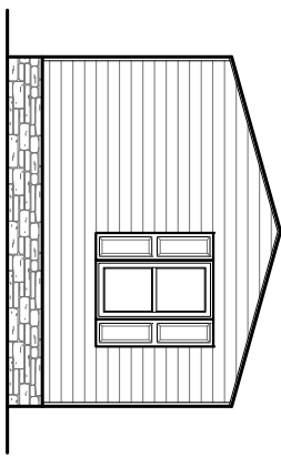
RIGHT SIDE ELEVATION OPT 56' HOUSE
