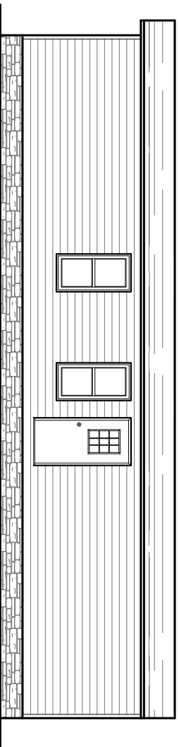
REAR ELEVATION
