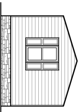
RIGHT SIDE ELEVATION
