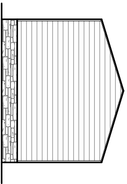
LEFT SIDE ELEVATION
