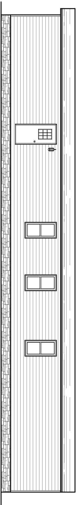
REAR ELEVATION
