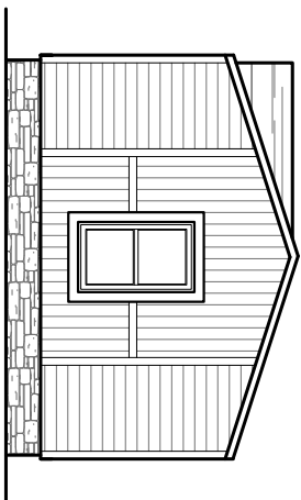
RIGHT SIDE ELEVATION
